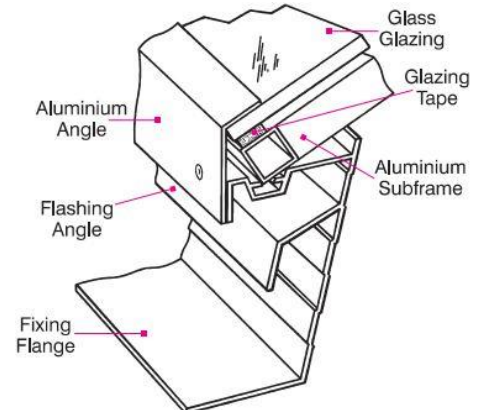
Cross Section of Glass Rainbowlite Pyramid with Aluminium Sub-frame for larger sizes
